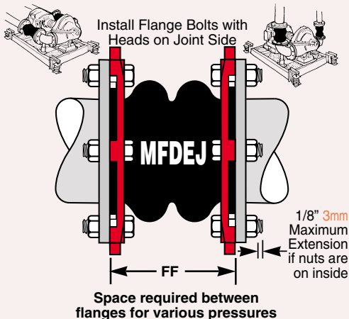
MASONFLEX MFDEJ Pressure Extension Table
